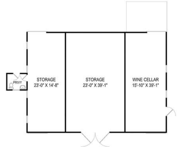
BARN FLOOR PLAN
