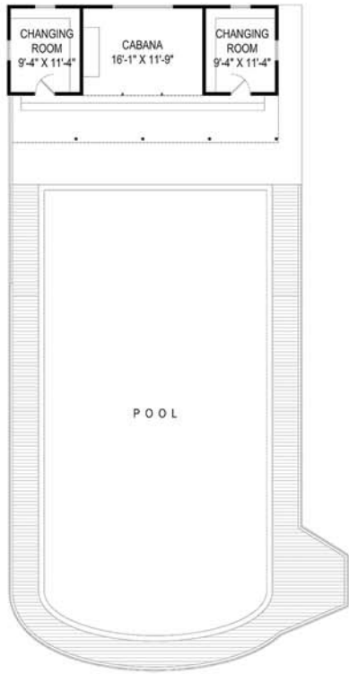
POOL HOUSE FLOOR PLAN
